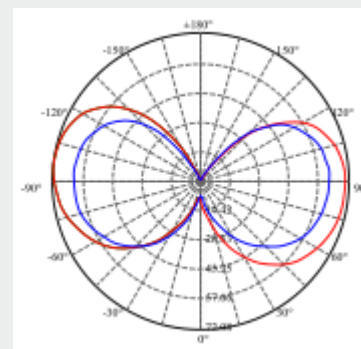
Peak of light intensity (max. cd)
